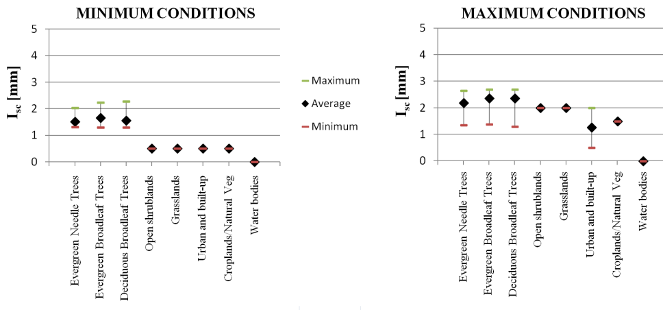
Figure 7. Earth observation based interception storage capacity estimates per land-cover class in the Upper Woluwe River catchment, under minimum and maximum vegetation conditions.
