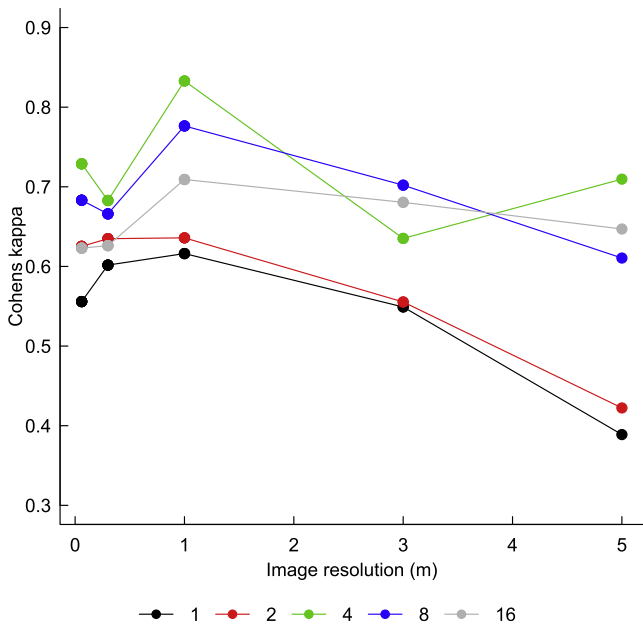
Fig. 7. Cohen's kappa coefficient plotted against image resolution for the different cluster sizes in each experimental treatment.
