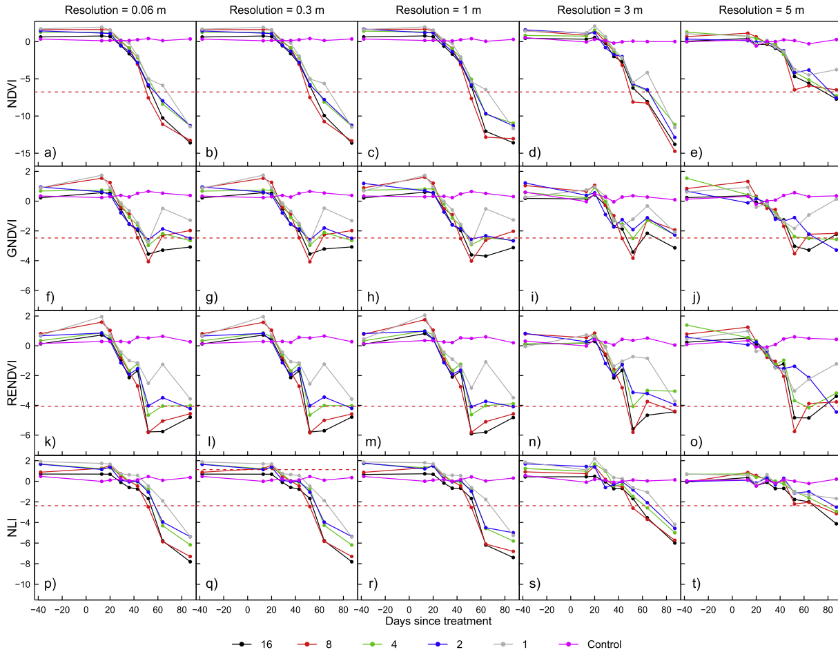
Fig. 6. Mean detrended spectral indices for clusters within the study area. Red dashed line show the 25th and 75th percentile of the pre-treatment spectral index. The area between the red-dashed line can be deemed a “no-change” region, a spectral index can be considered to have changed over time when its mean value moves outside of the no-change zone. (For interpretation of the references to colour in this figure legend, the reader is referred to the web version of this article.)
