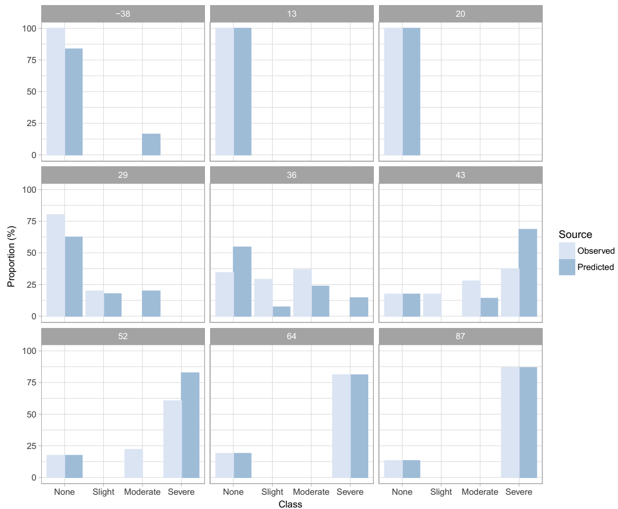
Fig. 5. Observed (field) and predicted (random forest) proportion of trees assigned to each stress class. Results are based on a 10% random resampling of the training dataset, this provides total separation of training and testing data and so is an independent validation. Each panel shows the results for a different time step, the number in the header refers to the number of days since treatment.
