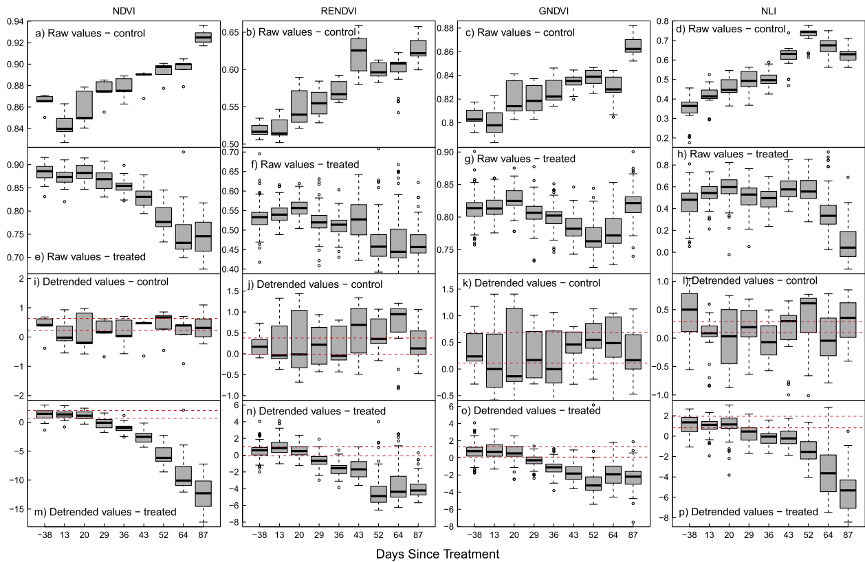
Fig. 3. Box and whisker plots showing the raw and detrended values for selected spectral indices observed in the control plots ( n = 5 ) and the treated plots n = 30 . Upper and lower red dotted lines indicate the extent of the “no-change” region. The no change region was defined as the 25th and 75th percentiles of the spectral value prior to herbicide treatment (30th October 2015). An area was classified as exhibiting significant stress if the 75th percentile of the spectral index value dropped below the no change region. (For interpretation of the references to colour in this figure legend, the reader is referred to the web version of this article.)
